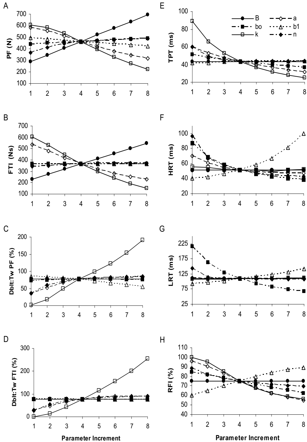
Figure 6 Representation of the parameter effects on simulated force characteristics for the 2 nd order nonlinear model. 2 nd order nonlinear model parameter effects on select force characteristics for the 10 Hz constant frequency pattern. Panel A: peak force (PF); B: force time integral (FTI); C: relative doublet PF; D: relative doublet FTI; E: time to peak tension (TPT); F: 1/2 relaxation time (HRT); G: late relaxation time (LRT); and H: relative fusion index (RFI, see text for operational definitions). Please see Table 2 for parameter baseline and increment values.
