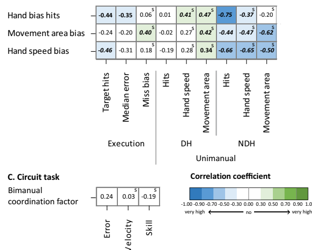
Fig. 6 Pearson and spearman’s rank correlation coefficients of the unimanual and task execution parameters with the bimanual parameters of the ball-on-bar task (A), object-hit task (B) and circuit task (C) for the selected parameters in children with uCP. DH dominant hand, NDH non-dominant hand, s spearman’s rank correlation
